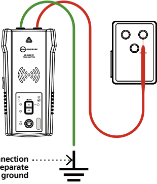
Separate ground connection (Preferred)
